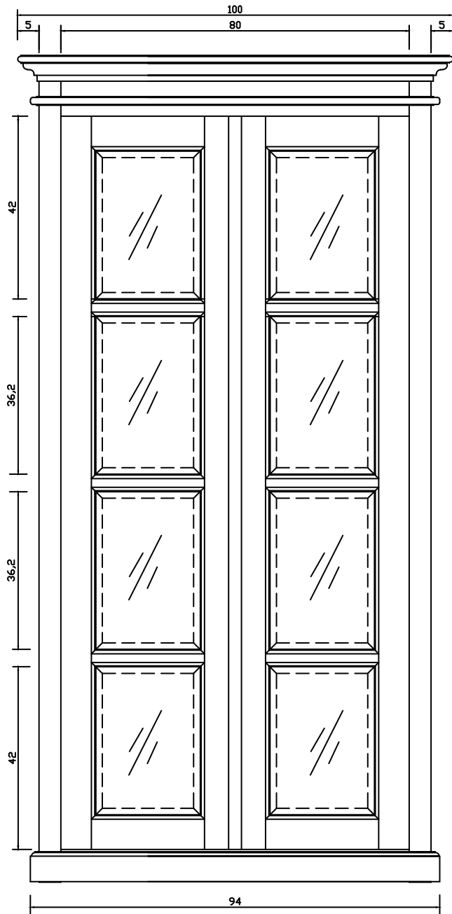
FRONT VIEW
