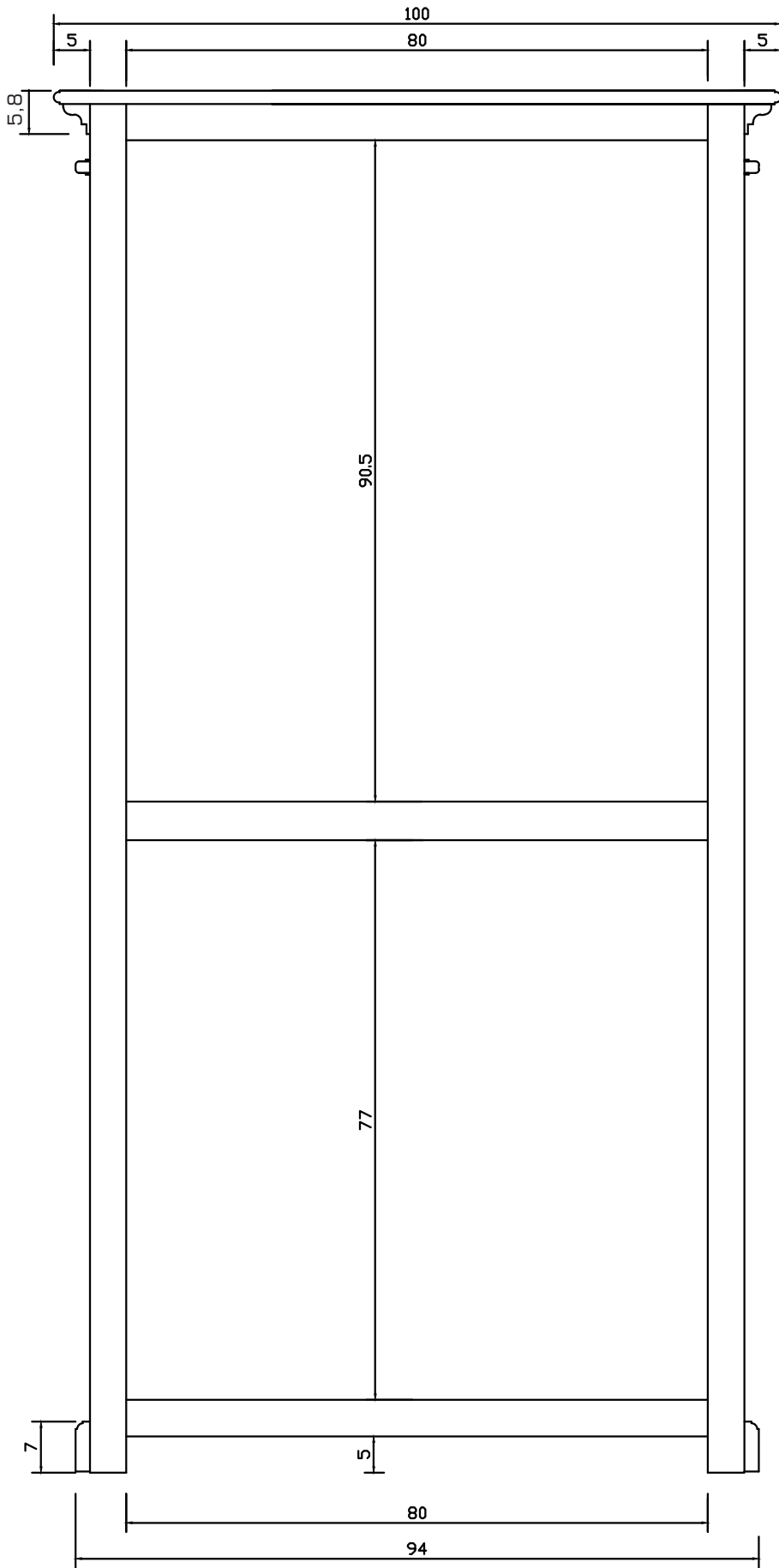
BACK VIEW
