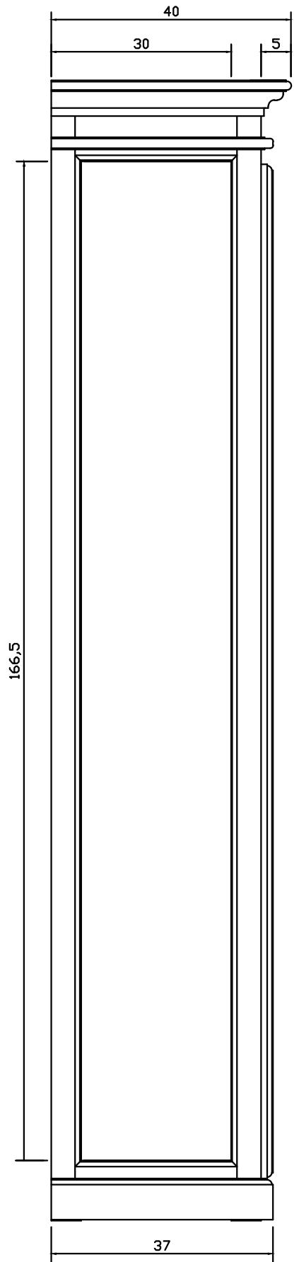
SIDE VIEW
