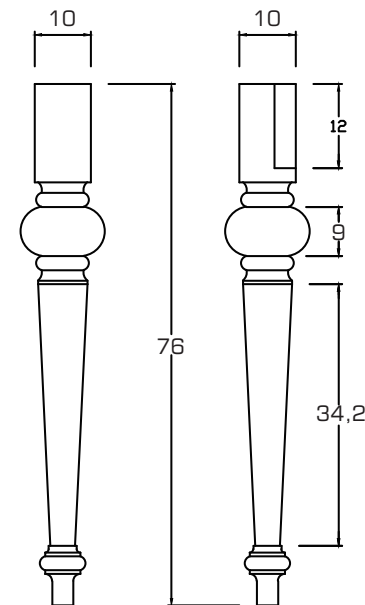
LEG DETAIL
